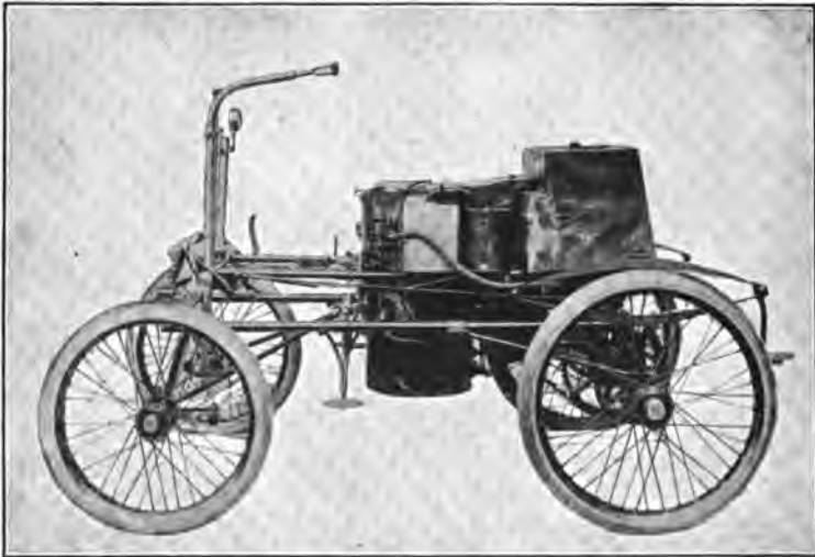
FIG. 272. —Underframe and Running Gear of the McKay Carriage, showing the position of the boiler and water tank. The gasoline tank in this carriage is inside the water tank, being thus entirely surrounded by water and protected from the fire. Contrary to the practice of most other American steam carriages, the engine is placed at the rear of the boiler, hence nearer the drive sprocket. The boiler structure seems longer than in most carriages, owing to the preheating coils, or waterleg, between the top plate of the burner and the base of the boiler.
